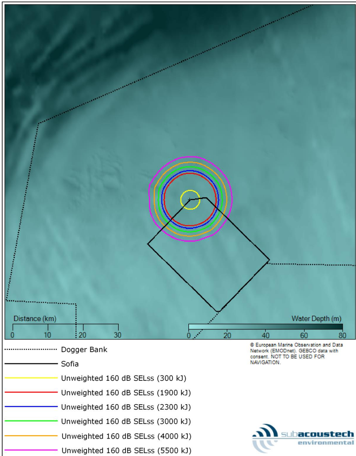
Figure B 4 Contour plot showing the unweighted 160 dB re 1 \mu\text{Pa}^2\text{s} \text{SEL}_{\text{ss}} impact ranges for possible avoidance of area in mid-frequency cetaceans for the six modelled hammer blow energies
